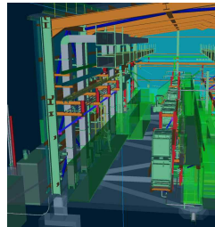
HVAC Modeling-2
